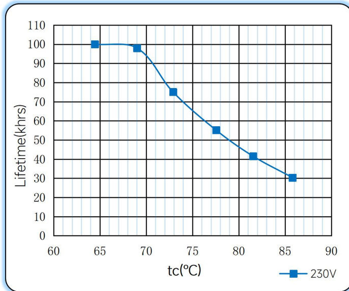
Lifetime vs. Ambient Temperature Curve
